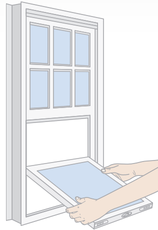
Remove Sash
